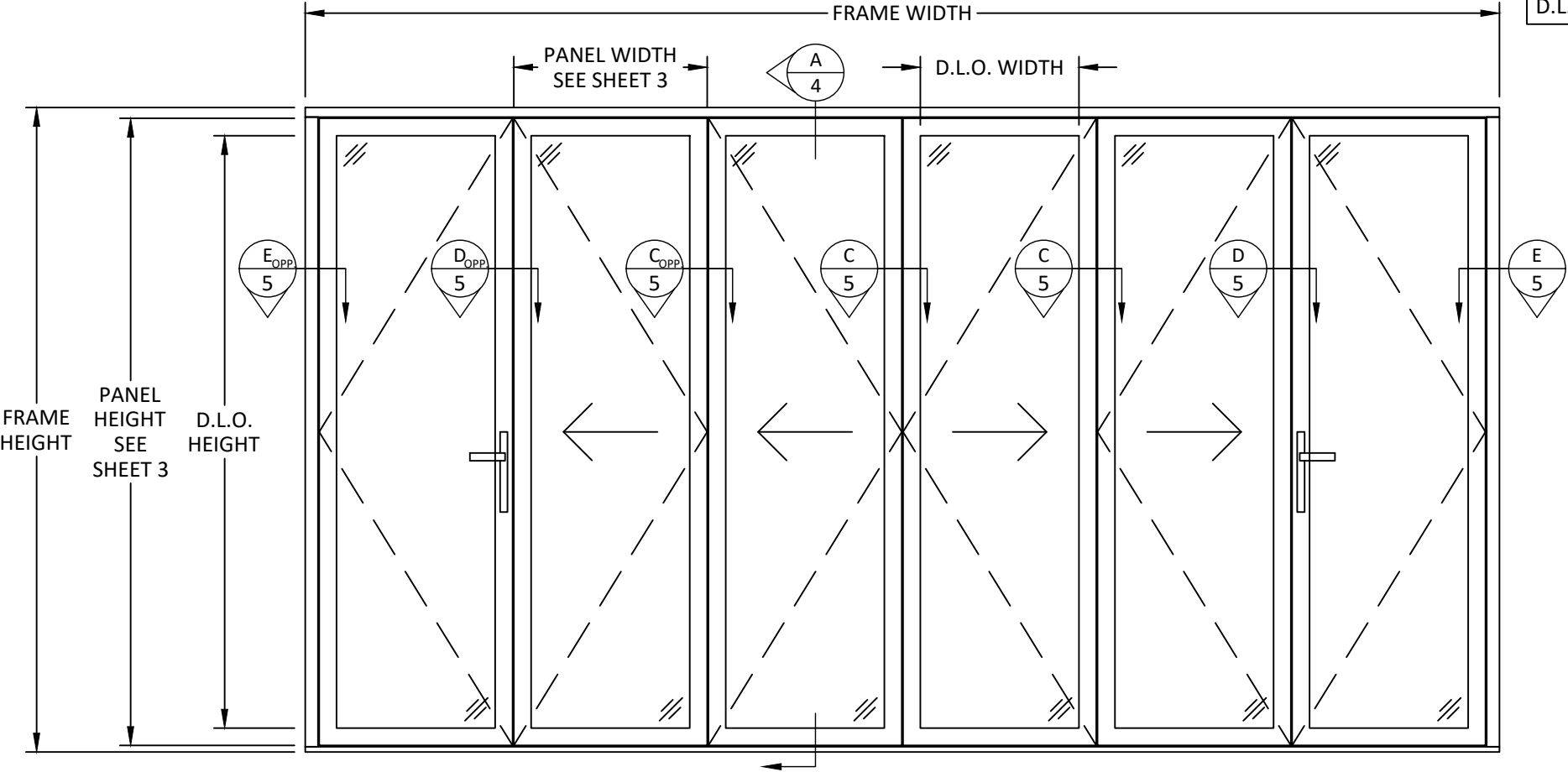
TYPICAL ELEVATION
